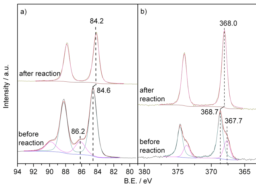
Figure 3: Au(4f) (a) and Ag(3d) (b) XP spectra of the NPG(Ag)-3 catalyst before and after 1000 min on stream.
